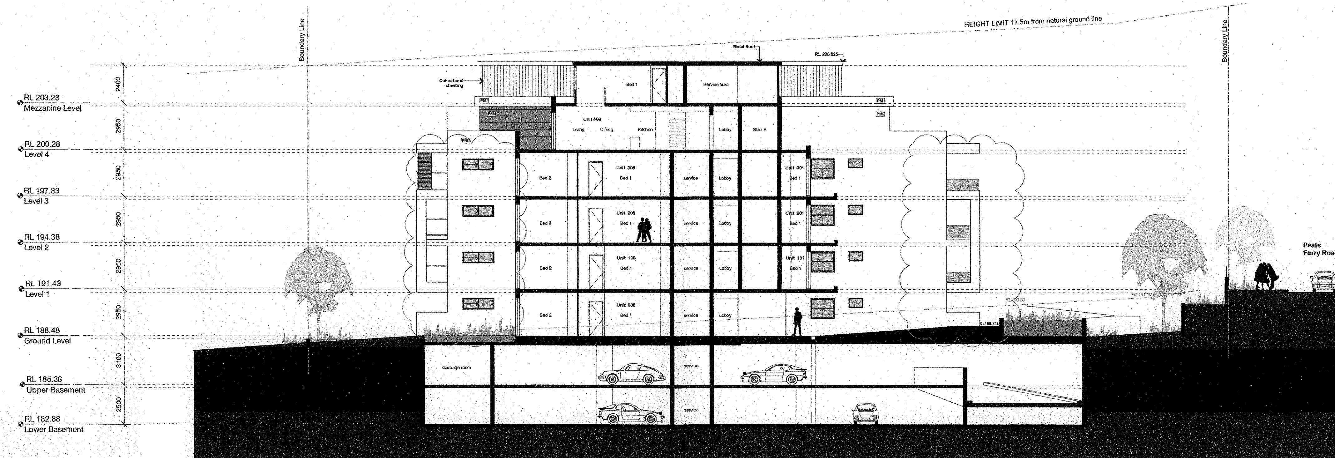
1 Section AA 1:150 @ A1
